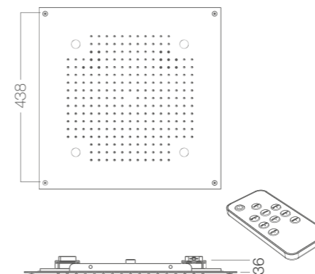
GY 477 ✓ L/H 470 mm ✓ G. 1/2" M
